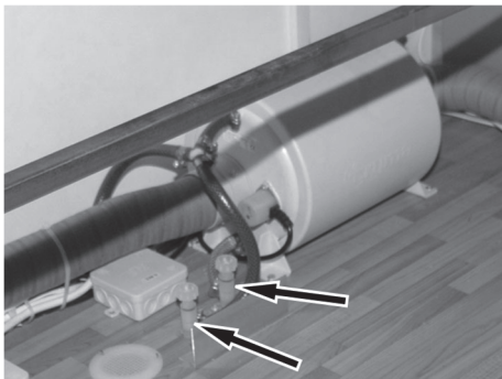
Abb. 149: Ablassventile
