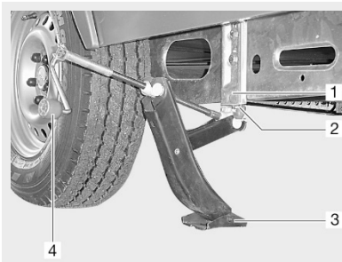
Fig. 176: Cric, AL-KO
